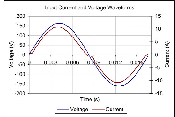
Input AC Current Waveform (ITHD = 16.83%, 50% Load)
