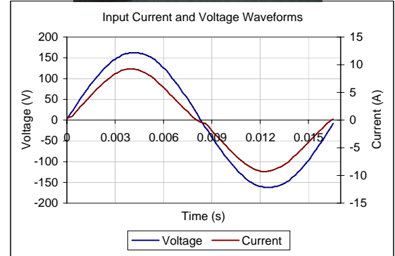
Input AC Current Waveform (ITHD = 15.06%, 50% Load)
